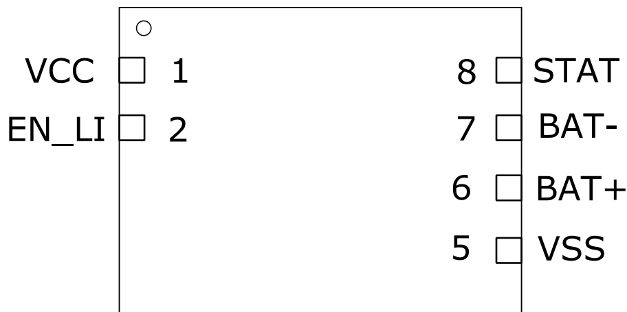
Pic.1 Schematic view ACM1803B.
