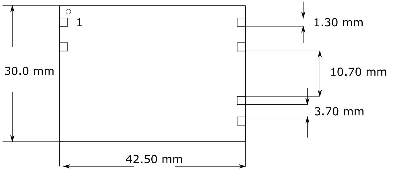
Pic. 7 Overall dimensions of the ACM1803B module.
