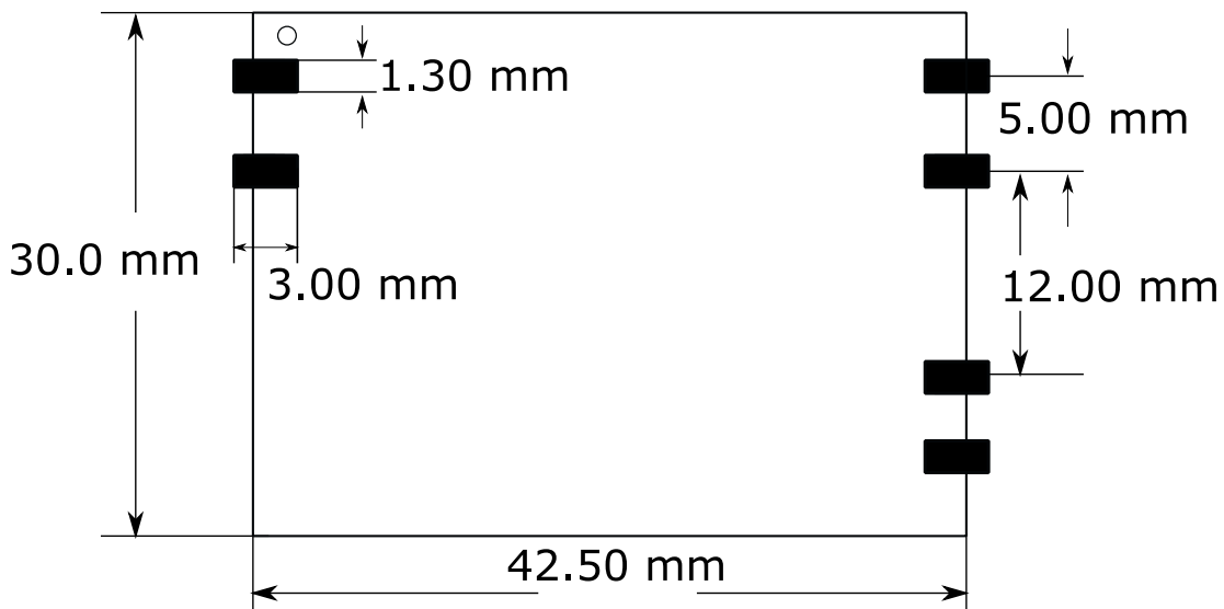
Pic. 8 Recommended mounting seat for ACM1803B module.
