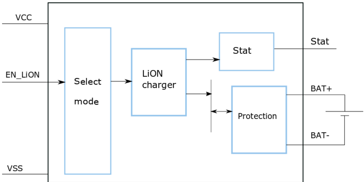
Pic.3. Main circuit nodes scheme ACM1803B.
